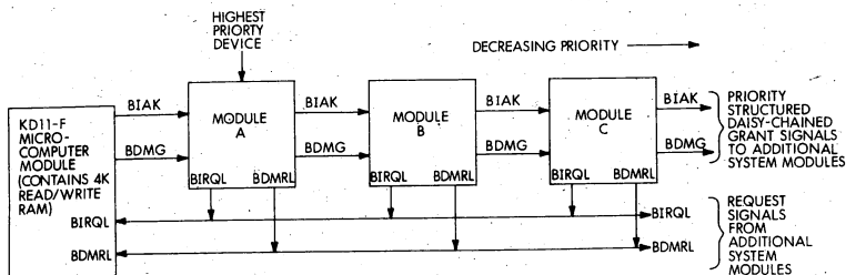
Figure 1-8 Bus Priority Structure
