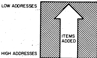
Figure 5-1: Stack Addresses
