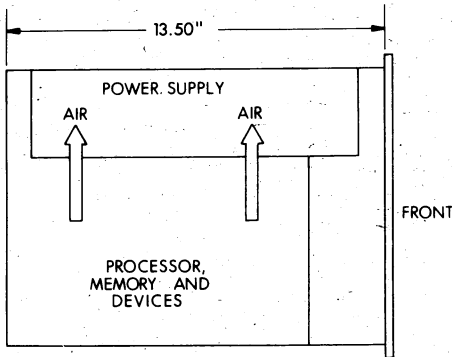
Figure 2-2 PDP-11/03 Assembly Unit
