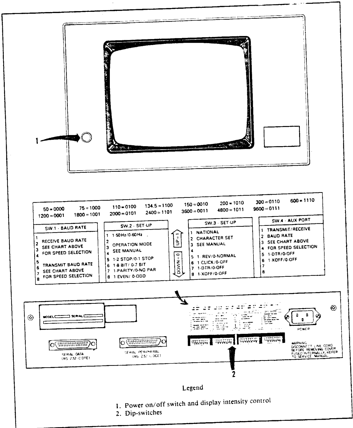
Figure 3-1 Operating Switches and Controls
