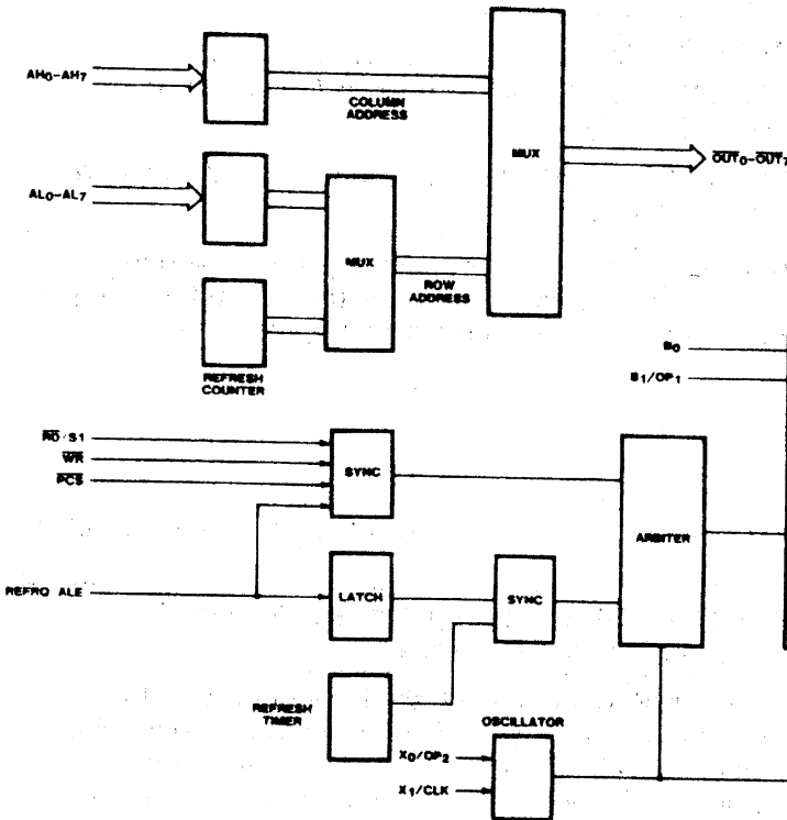
Figure 1. 8203 Block Diagram
