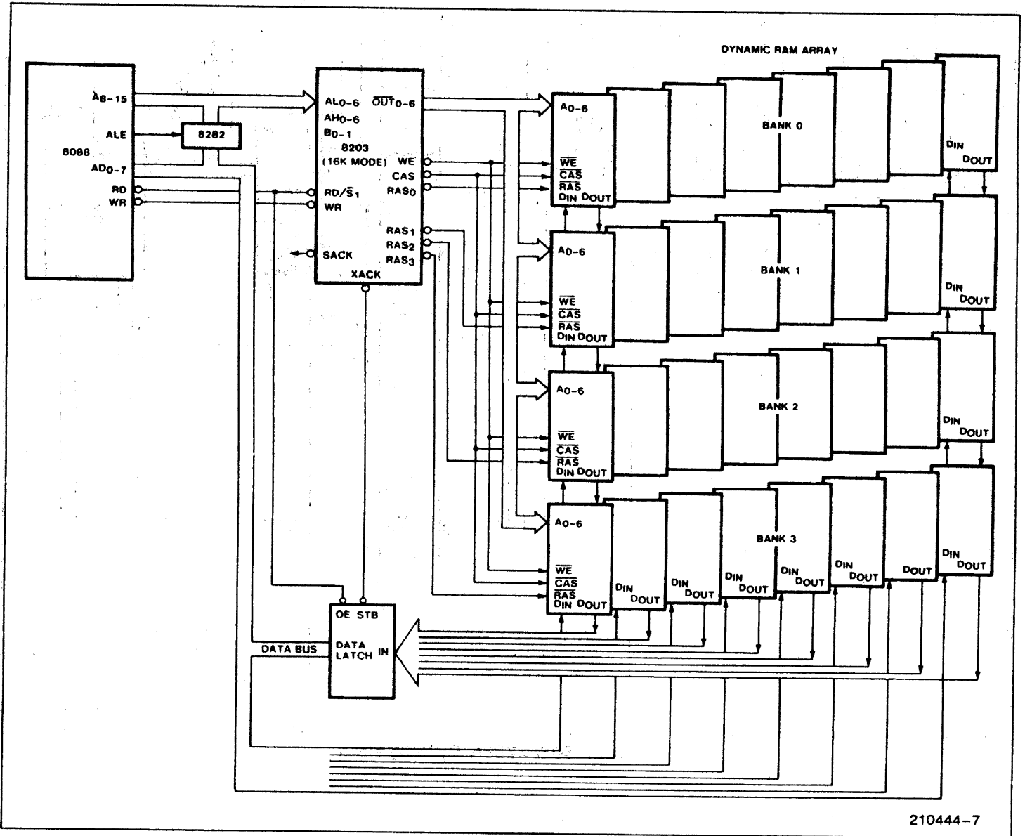
Figure 10. Typical 8088 System
