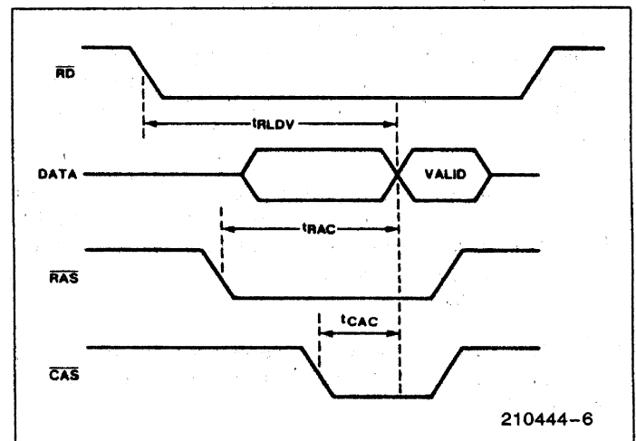
Figure 9. Read Access Time
