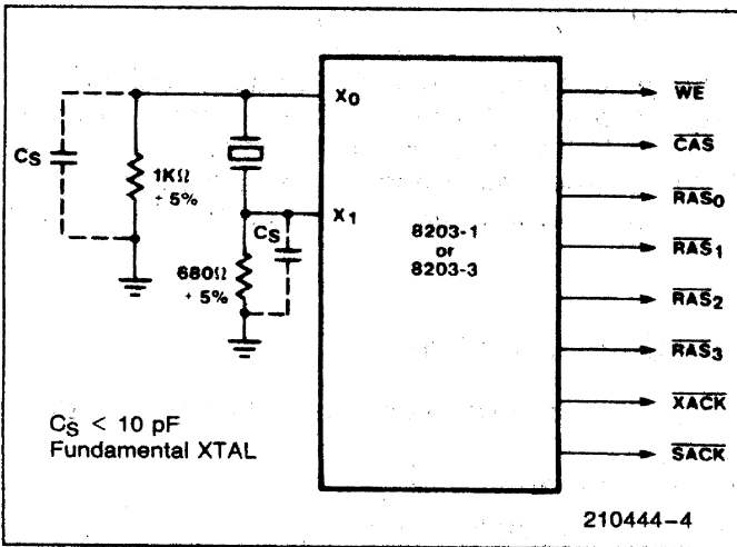
Figure 3. Crystal Operation for the 8203-1 and 8203-3
