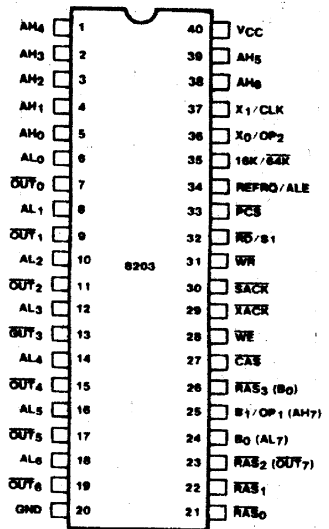
210444-2 Figure 2. Pin Configuration
