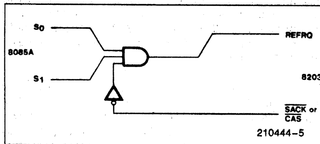
Figure 7. Hidden Refresh
